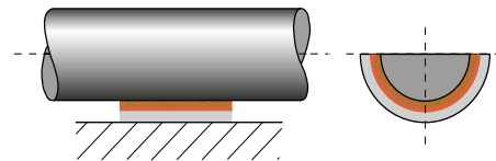
Fig. 26: Boundary lubrication
