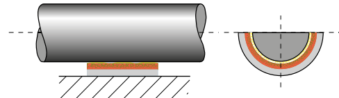
Fig. 25: Mixed film lubrication
